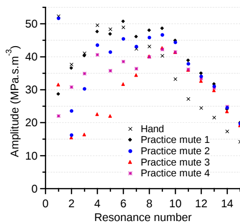
Figure 10. Amplitude of resonance peaks for valve 1, Bb horn with hand in bell and four different practice mutes in bell. (Error bars typically within size of symbol).
