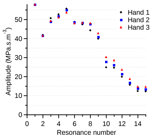
Figure 6. Amplitudes of resonance peaks for an open Bb horn with three different hands in the bell. (Error bars typically within size of symbol).
