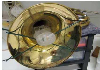
Figure 2. Replica hand in (rotated) playing position in the bell of the horn.
