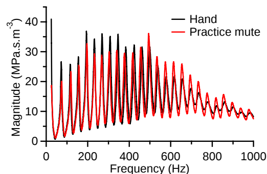
Figure 9. Impedance spectra for valve 1, F horn with hand in bell and practice mute in bell.
