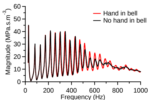
Figure 4. Impedance spectra for the open F horn with and without hand in bell, illustrating the effect of the hand on the cutoff frequency of the bell.
