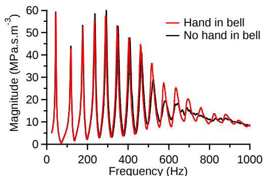
Figure 5. Impedance spectra for the open Bb horn with and without hand in bell.
