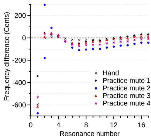
Figure 11. Variation in frequency of resonance peaks from harmonicity for valve 1, Bb horn with hand in bell and four different practice mutes in bell. (Error bars within size of symbol).
