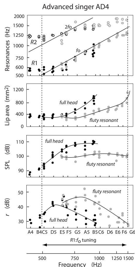
FIG. 7. Comparison of vocal tract resonances R1 and R2 , lip articulation, sound pressure level (SPL) and the difference r in harmonic level [defined by Eq. (1)] between “full head” (black symbols) and “fluty resonant” (gray symbols) productions by advanced singer AD4. See caption to Fig. 4 for further details.
